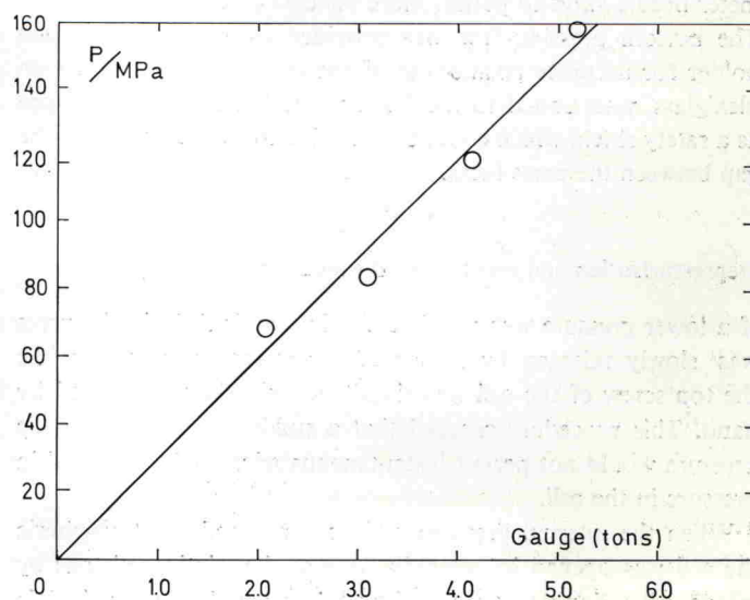
Fig. 2. Pressure calibration of the circular dichrometer cell based on the compression of water showing P vs. gauge readings.
